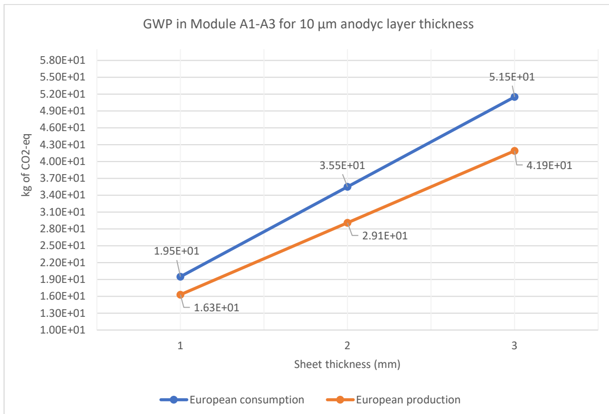
Figure 2 Sensitivity analysis: EU consumption GWP against EU production GWP
